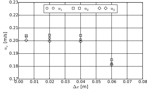
(c) Convergence of velocities at three different locations behind the porous sheet over \Delta x .
