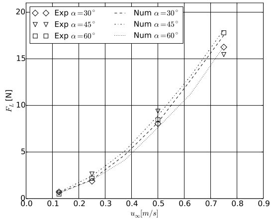
(b) Lift forces over inflow velocity.
