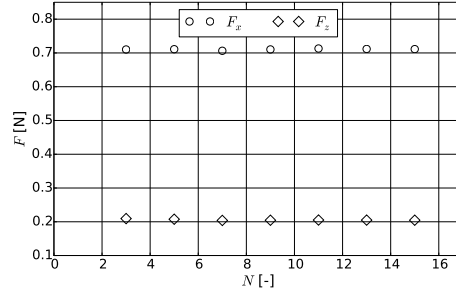
(b) Convergence of global forces over N .
