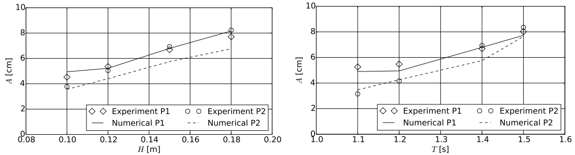
(a) Maximum deformation of the sheet for different wave heights and T = 1.4 s. (b) Maximum deformation of the sheet for different wave periods and H = 0.15 m.
