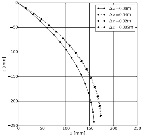
(e) Convergence of deformation over \Delta x .
