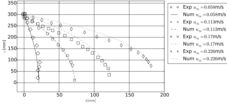
(c) Distribution of the deformed centre line for different inflow velocities.
