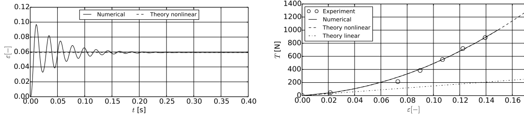
(a) Example for the convergence of the elongation \varepsilon over time t .
