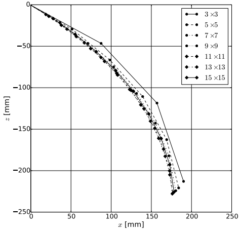
(f) Convergence of deformation over N .
