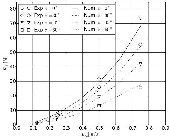
(a) Drag forces over inflow velocity.
